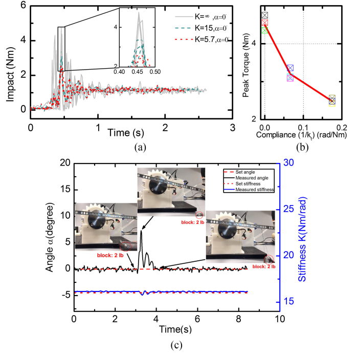
Fig. 10. Behavior shaping tests. (a) Passive impact reduction test results. The joint torque compared between a fixed joint at \alpha = 0^\circ and a joint with a preset stiffness of K = 15 . The peak impact torque could be reduced by 40%, but without the active angle control, the joint angle could not be restored. (b) Relations between the stiffness and impact. (c) Hybrid control with passive stiffness and active regulation; disturbance could be restored by returning to the original angle.
