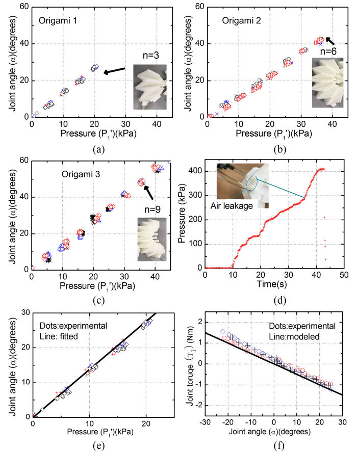
Fig. 6. Origami chamber static test results. (a–c) Performance repeatability test: Origami 1, Origami 2, and Origami 3. Each test was repeated three times. (d) Maximum withstanding pressure of the origami chamber. (e), (f) k calibration and validation tests.
