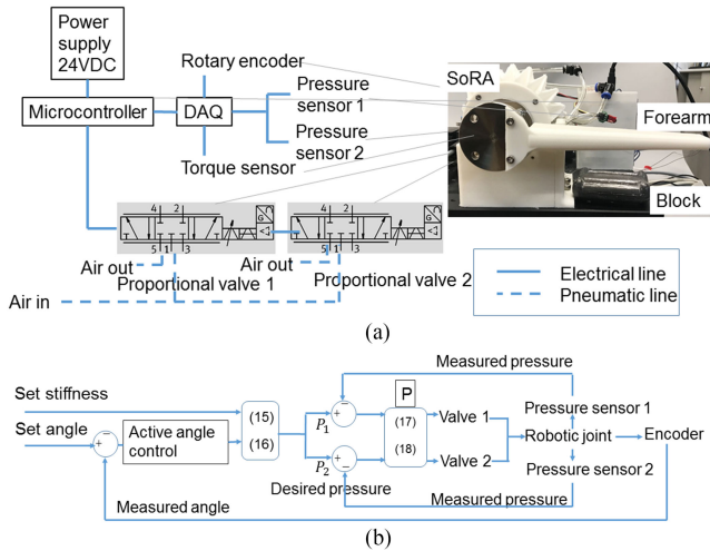
Fig. 8. (a) Schematic of the control system with hardware. (b) Control block diagram of the joint system.
