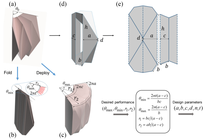
Fig. 2. Concept of the origami chamber. Three working states: (a) NS, (b) FF state, and (c) FD state, together with the (d) geometrics of one unit in the NS and (e) form of the flat sheet.
