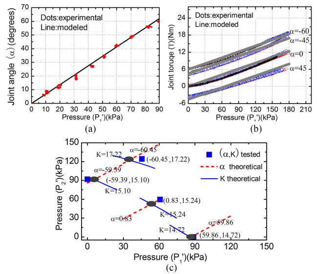
Fig. 7. SoRA static test results. (a) SoRA free-space test. (b) SoRA static torque test. (c) SoRA variable stiffness test. Solid squares with illustration denote the actual angle and stiffness at given pressures. The modeled results corresponding to the experimental results are indicated as follows: \alpha : dash line, K : solid line, and intersecting circles: modeled results.
