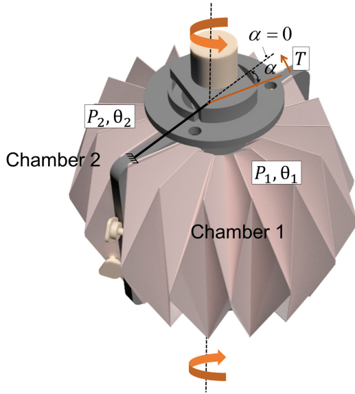
Fig. 1. Concept of SoRA with pressure sensor and encoder embedded. Chambers' pressure P_1 , P_2 , chambers' central angles \theta_1 , \theta_2 , and joint angle \alpha are illustrated.
