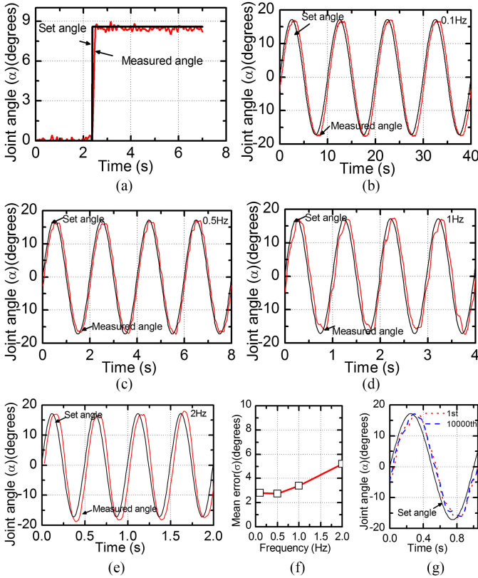
Fig. 9. Controller tests. (a) Step response test results. (b–e) Sinusoidal test results for 0.1, 0.5, 1, and 2 Hz. (f) Angle mean error at the tested reference signal frequencies. (g) Cycling test results showing the sinusoidal function following performance before and after the cycling test.
