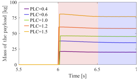
Fig. 5. The mass of the payload identified in this experiment. Payload varies from 20kg to 75kg. Payload varies from 20kg to 75kg, which corresponds to PLC (Payload Capacity) from 0.4 to 1.5. The identification starts from 6 s (red region) and ends at around 6.5 s (blue region)
